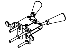
REF. B-106 / B-107 HANDLE CLAMPS
